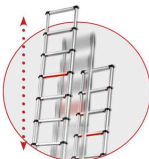
Unit has a flange in the legs which restricts air flow and therefore gives controlled retraction to compact the unit smoothly from 3810mm to 910mm
